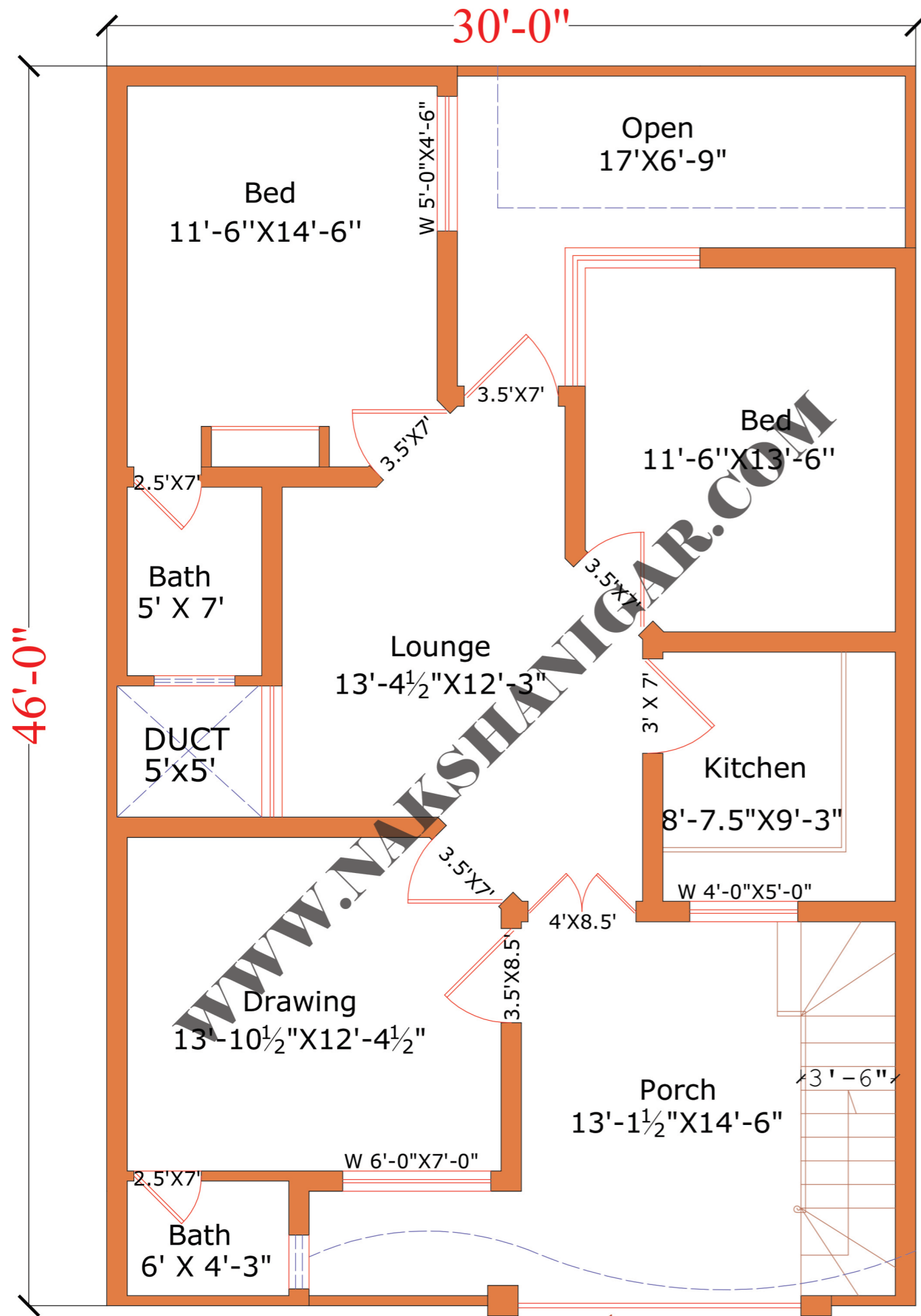
GROUND FLOOR PLAN Covered Area: 1240 SFT
